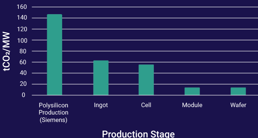
Solar Supply Chain CO 2 Emissions By Production Process
