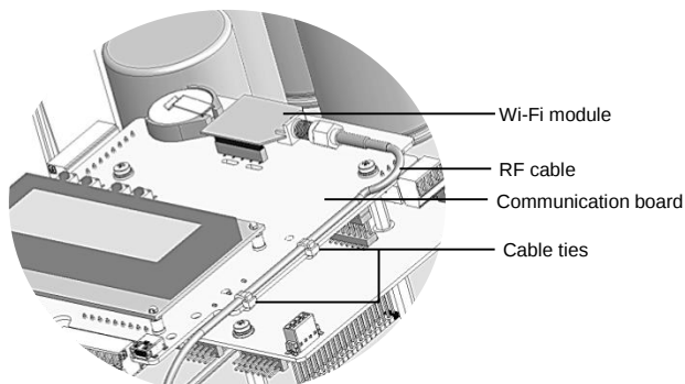
Figure 6: Wi-Fi and RF cable on the communication board
